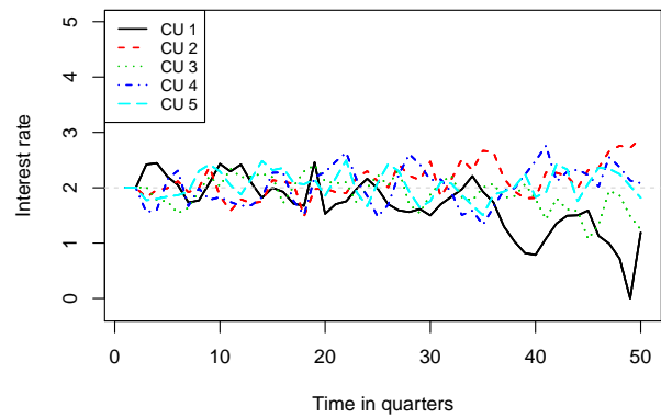
(f) Interest rate, \Phi_\pi = 6 and \Phi_y = 2
